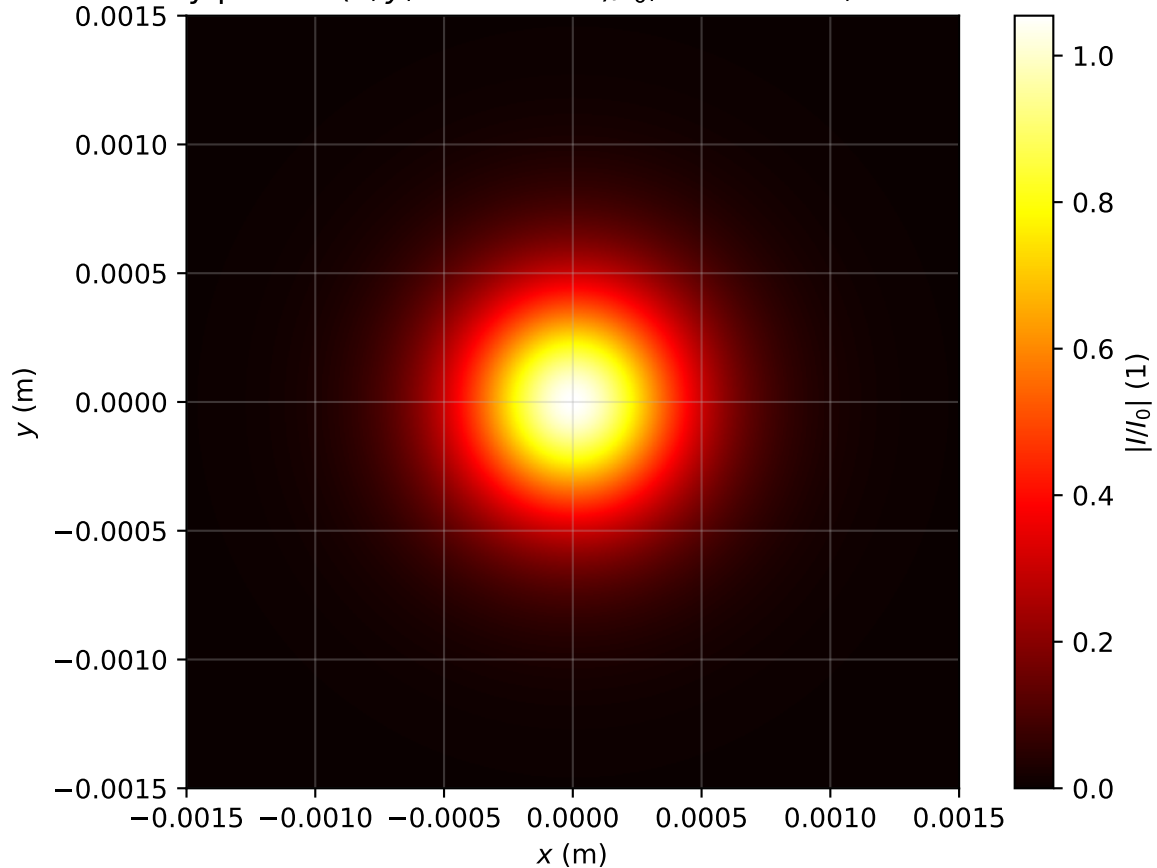
Intensity profile I(x, y, z = 3.184m)/I_0 , P_{in}=0.8P_{cr} , artificial time
